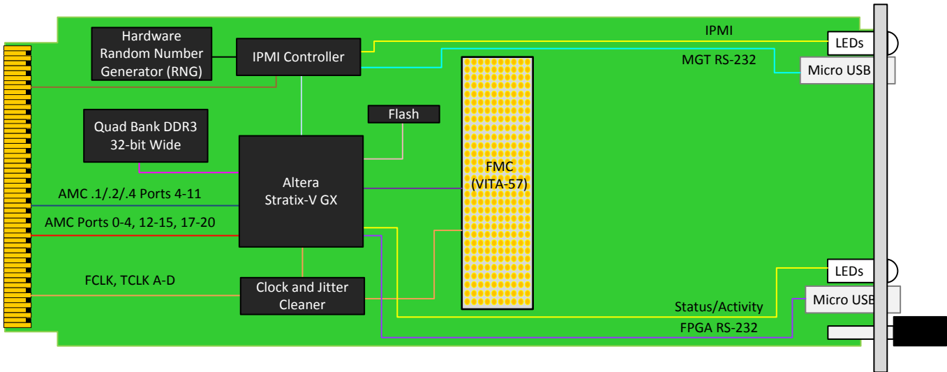
Figure 1: AMC532 Functional Block Diagram
