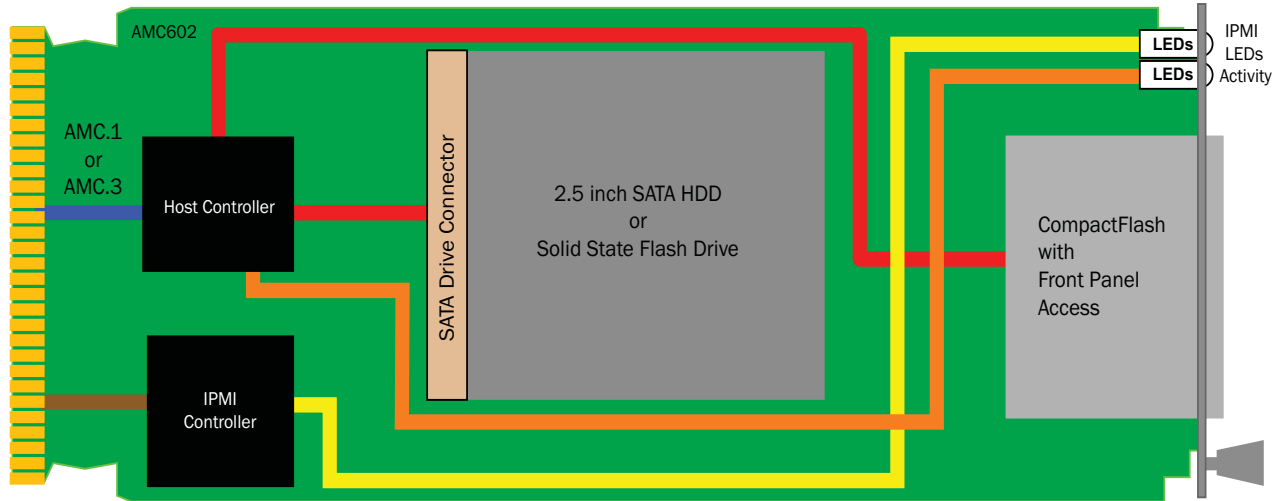
FIGURE 1. AMC602 Functional Block Diagram
