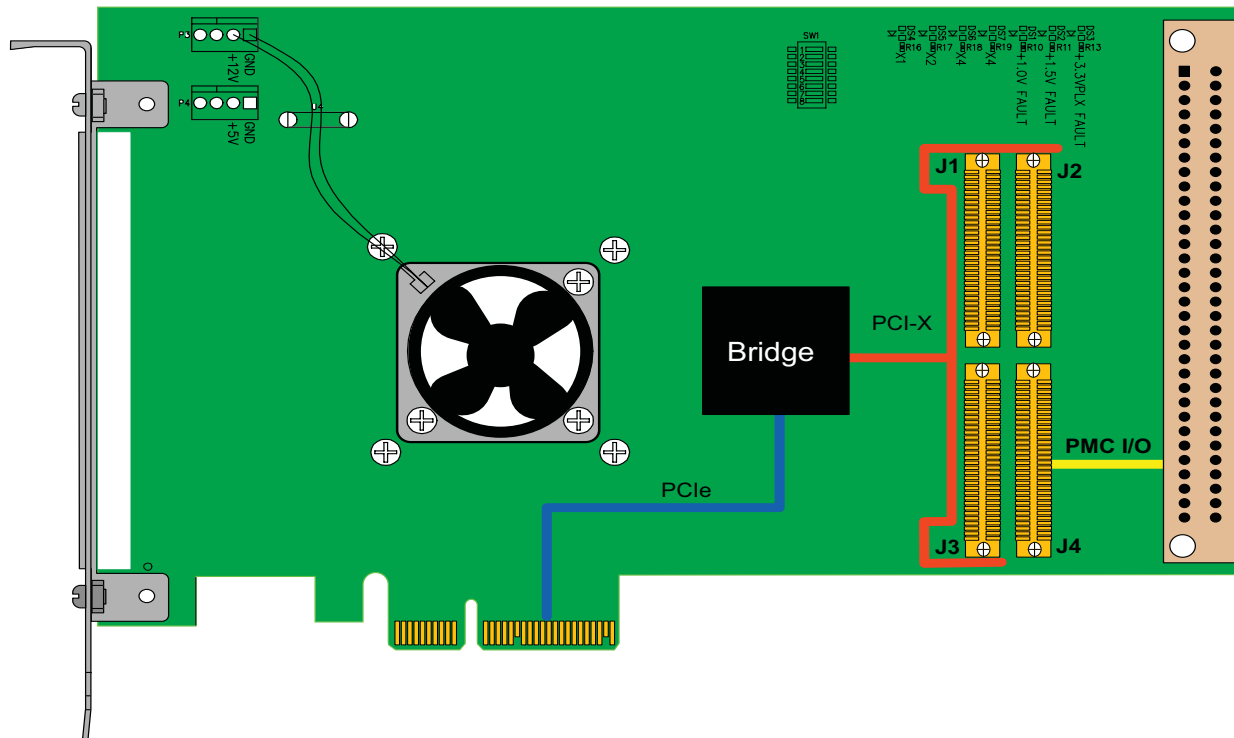
FIGURE 1. PCI104 Functional Block Diagram
