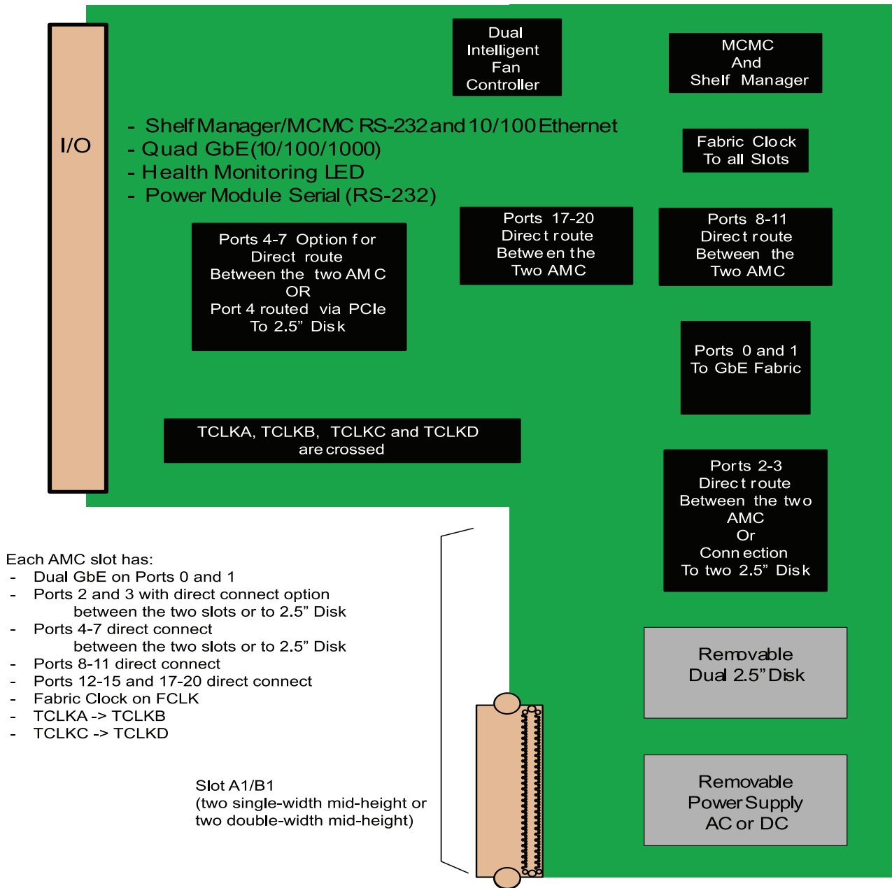
FIGURE 1. VT855 Functional Block Diagram
